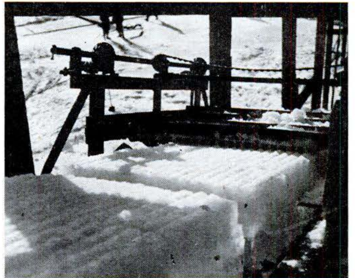
7. As the individual cakes move up, a planer shaves off slush and gives a rough surface to the ice for easier handling. Fourteen-inches of ice produce cakes weighing 322 pounds.
